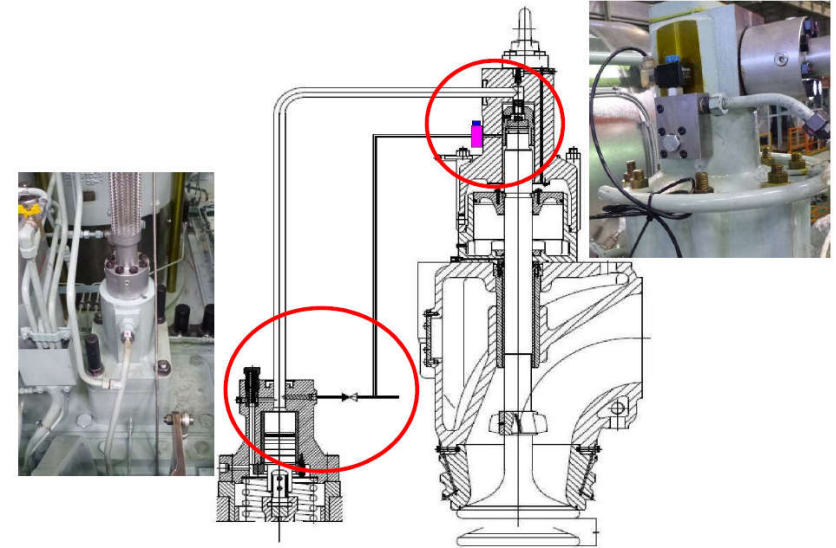
Eco Cam (TDP-042)
