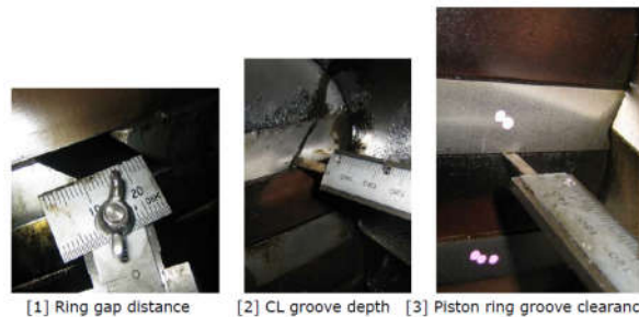
Piston Inspection Gauge (TN063)
