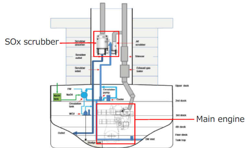
Signal / TC modification for SOx Scrubber (TN099)
