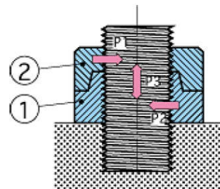
Anti-loosening Function for Camshaft Coupling (TN076)
