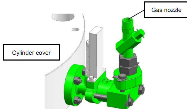
Back Seat Type Indicator Valve (TN102)
