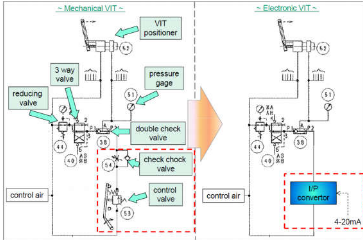
Electronic control VIT (TDP-041)
