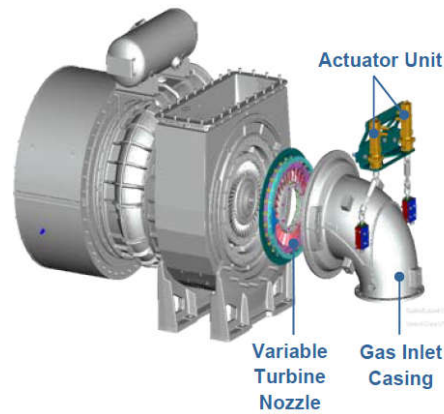
Variable Turbine Area
