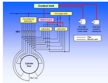
Alpha Lubricator System (TN029) *LO saving
