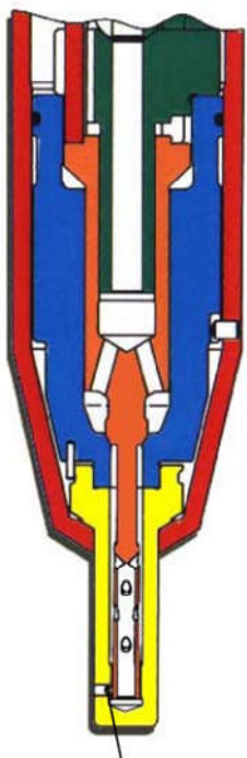
Slide Fuel Valve (TN037)
