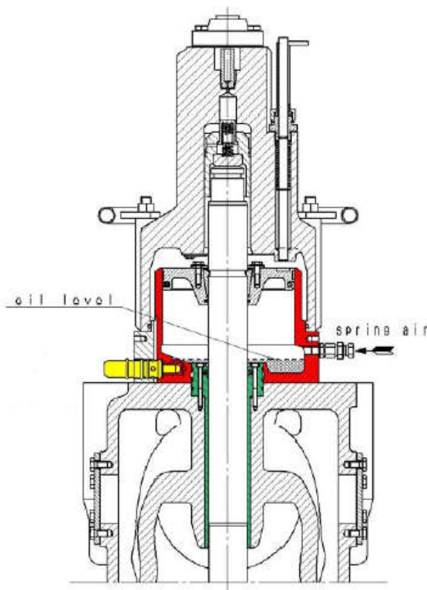
Controlled Oil Level sealing system (TN066)
