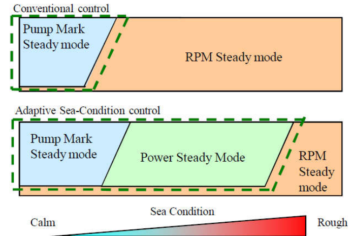
Adaptive Sea-Condition Control
